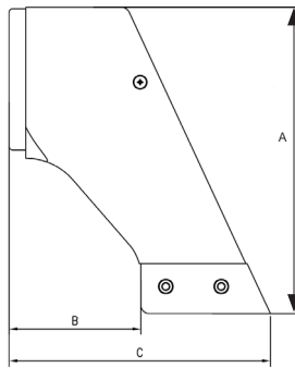
Square Drive Reaction Sleeve with Foot
